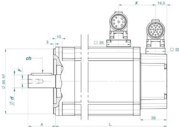
Power connector 4+4 PIN M23 turnable BEDC 110 - Signal connector 17 PIN M23 turnable AEDC 139
